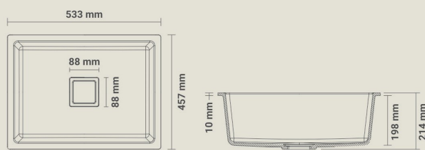
QTZ-104 Single Bowl Sink Brown Size : 21"x18" Weight : 11kg. Approx
