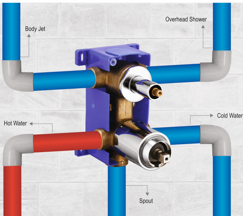
DCP-106 Concealed Body Single Lever Three outlet Diverter
