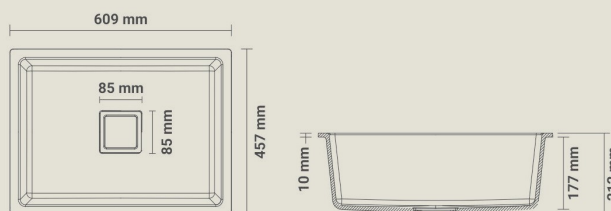
QTZ-105 Single Bowl Sink White Size : 24"x18" Weight : 12kg. Approx
