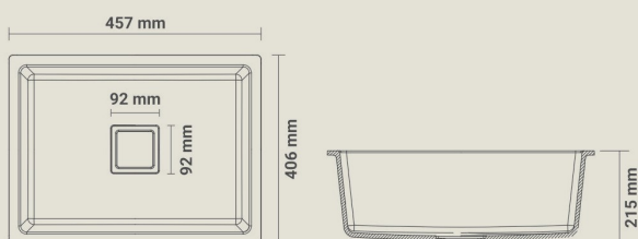
QTZ-103 Single Bowl Sink Black Size : 18"x16" Weight : 9kg. Approx
